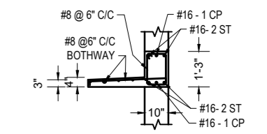
DETAILS OF ENTRANCE LOBBY LINTEL & CHAJJA SCALE:- 4'-0"=1"
