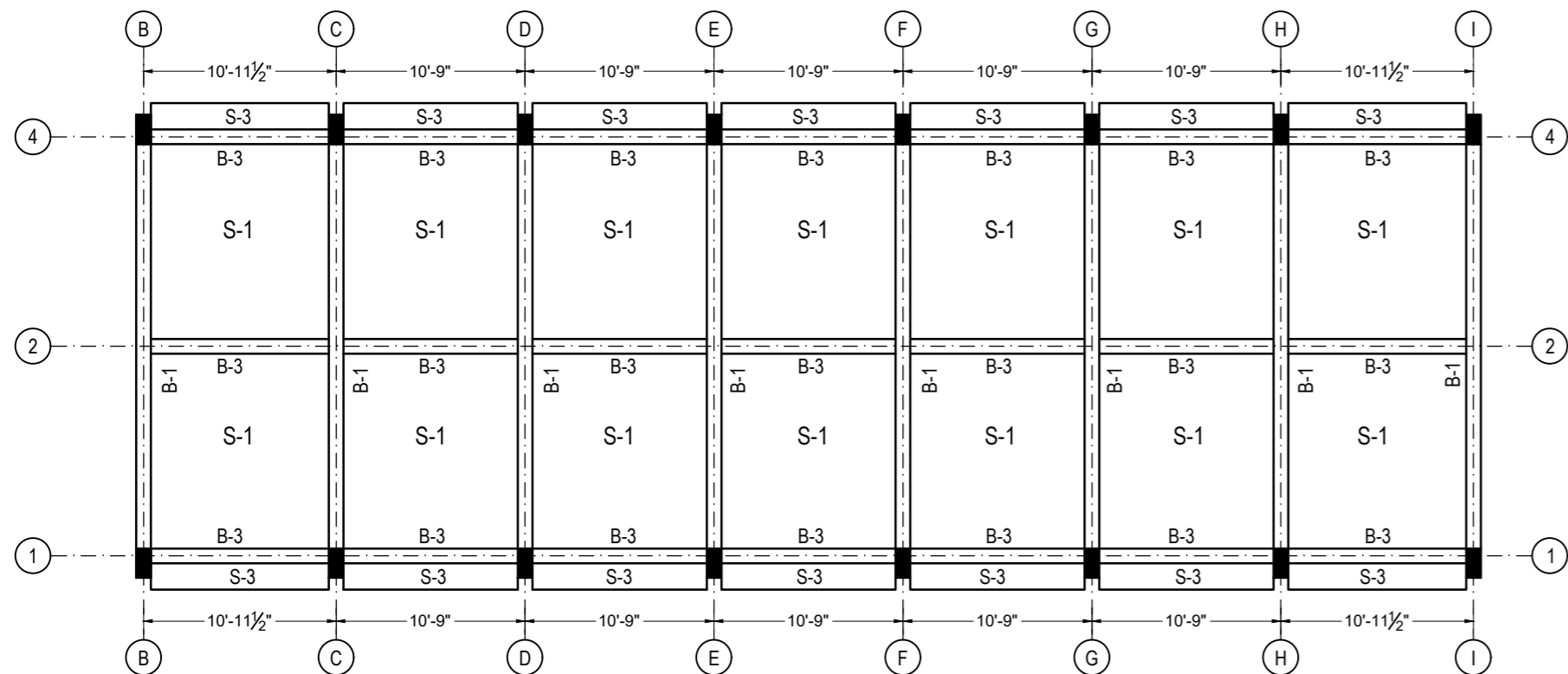
ROOF SLAB BEAM GRID PLAN SCALE:- 8'-0"=1"
