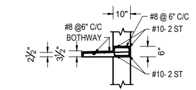
DETAILS OF LINTEL & CHAJJA SCALE:- 4'-0"=1"
