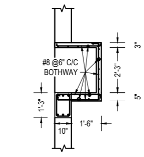
DETAILS OF CUPBOARD SCALE:- 4'-0"=1"
