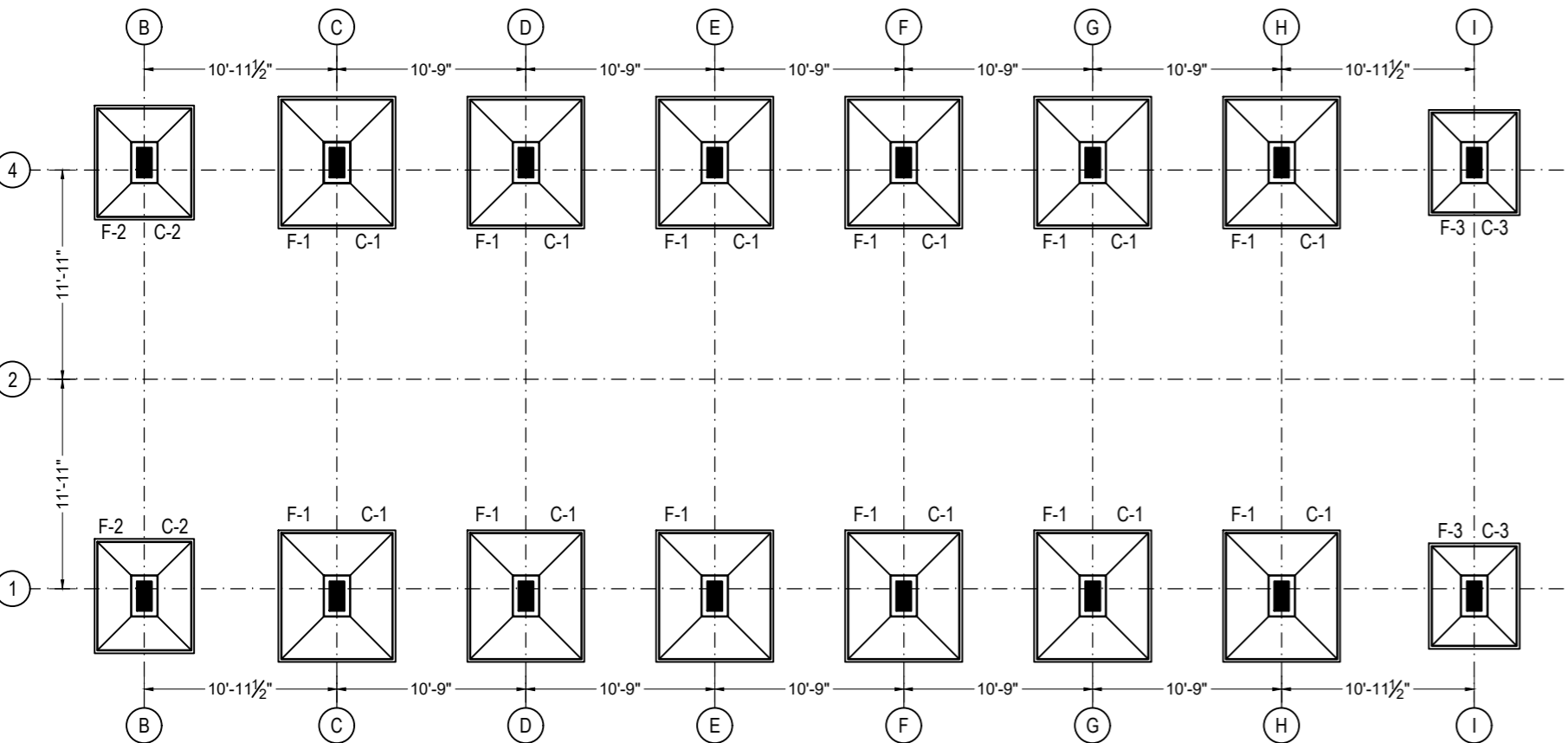
LAYOUT PLAN SCALE:- 8'-0"=1"
