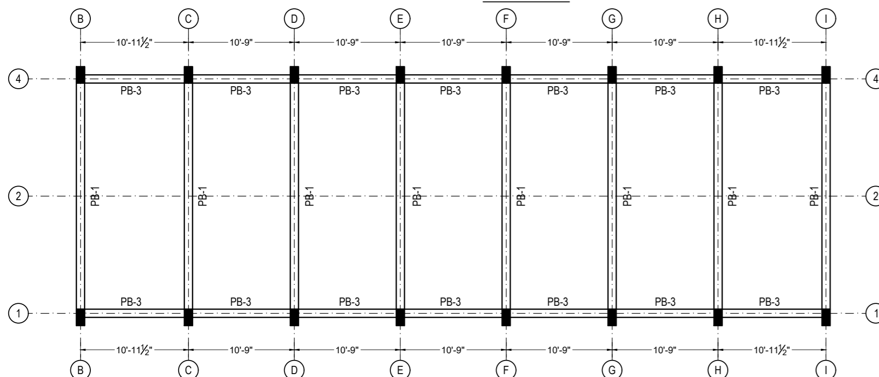
COLUMN TIE BEAM GRID PLAN SCALE:- 8'-0"=1"
